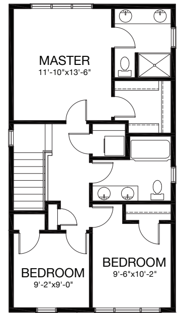
SECOND FLOOR = 740 SQ.FT.
